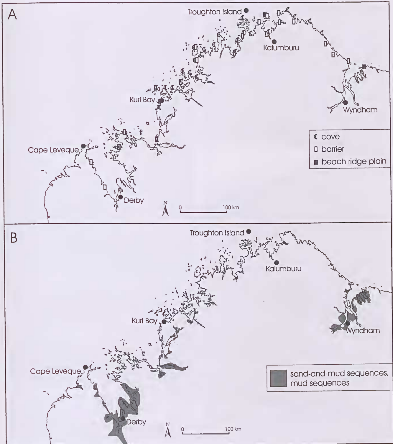
Figure 5. Maps showing occurrences of sandy coves, sand barriers, and beach ridge plains in the wave exposed outer margins of the ria coastal system, and both the sand-and-mud systems and mud systems are in the interior of embayments and gulfs.
